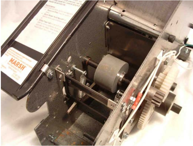
Fig 18 Cutter Arms
